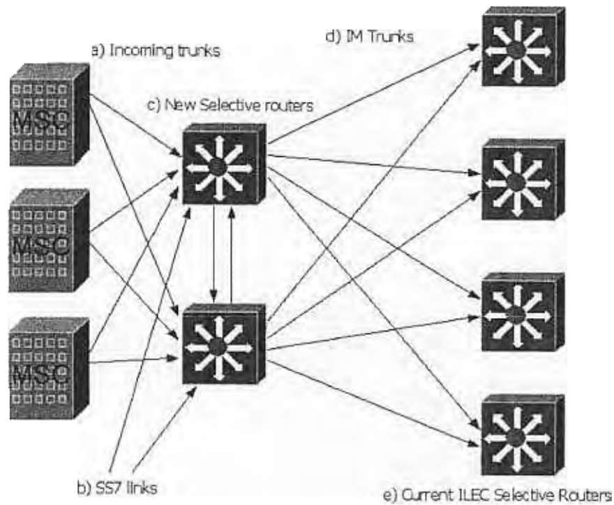
Figure 1.2 - Basic G-1 configuration
